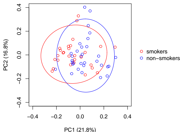
Ordination based on Bray–Curtis distance
